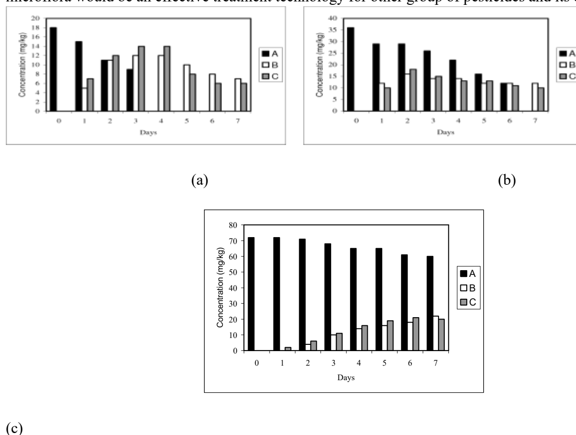
Figure 4. Concentration of intermediates found during the bioremediation of Fenvalerate amended soil (a) 25 mg/l Fenvalerate amended soil (b) 50 mg/l Fenvalerate amended soil (c) 100 mg/l
