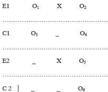
Figure 1. Solomon Four Non-Equivalent Control Group Research Design Key
