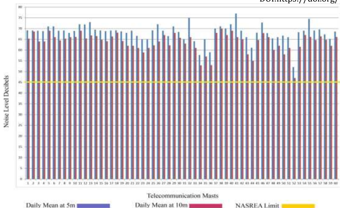
Figure 3: Measured Night Time Noise Level.
