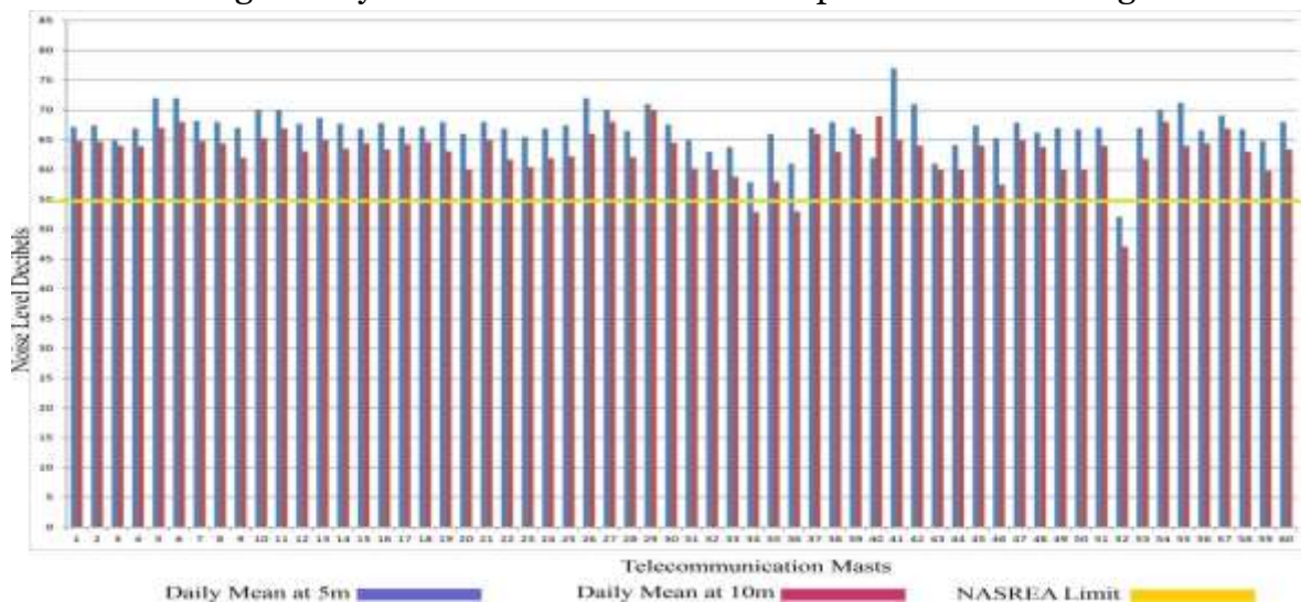
Figure 2: Measured Day Time Noise Level.
