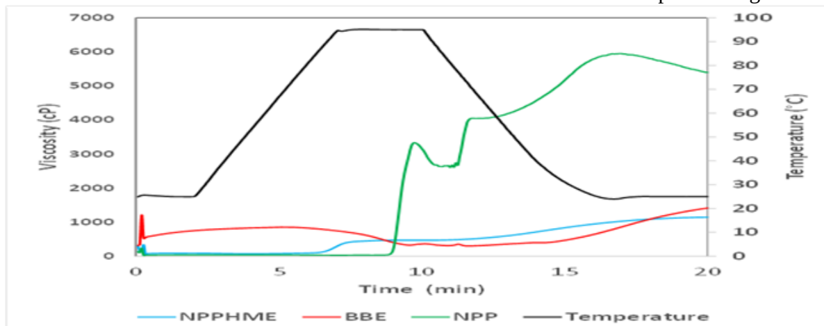
Figure 3: Pasting profile of native pigeon pea (NPP), extrudates from high moisture nontreated native pigeon pea (NPPHME) and low moisture alkaline treated (BBE) feed.
