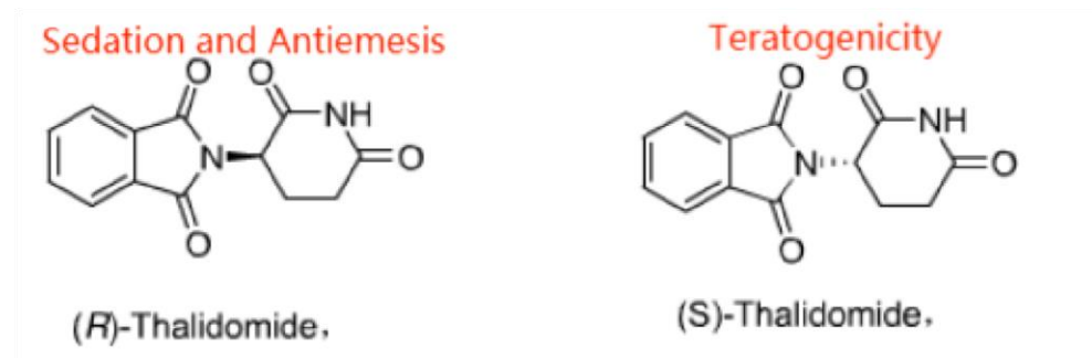
Figure 1: Two Molecular Structures of Thalidomide.
