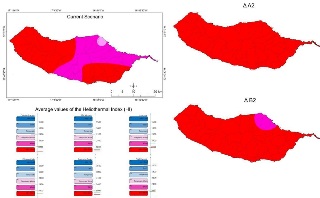
Figure 3. Interpolation of the Heliothermal Index (HI), for the current scenario and for the \Delta A2 and \Delta B2 scenarios proposed by Madeira Climate Strategy for 2070-2099
