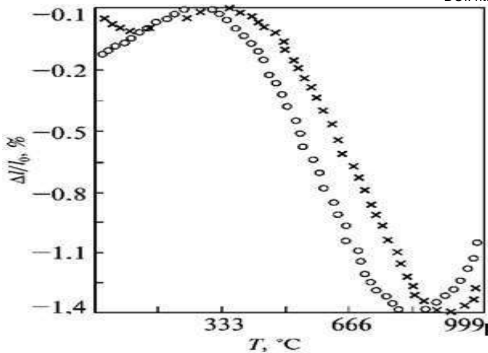
Figure 5. Dependence of relative thermal deformation of glass plastic on temperature (numerical experiment) at heating rates of °C/min, x – 25; o – 75.
