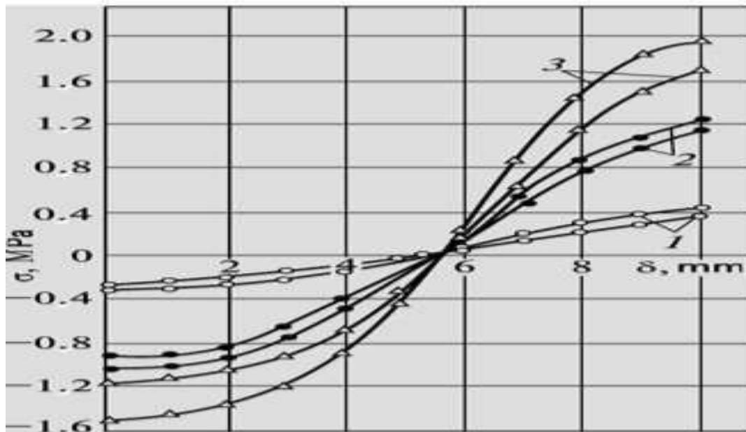
Figure 10. Distribution of stresses in samples from fiberglass in onesided heating: 1 (o) - t = 1.5 min; 2 ( \square ) - t = 2 min; 3 ( \square ) - t = 3 min (continuous curves – straightened sample; non-continuous – bent)
