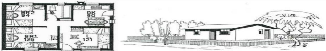
Figure 2: Perspective and plan of the NE 51/9 housing model
