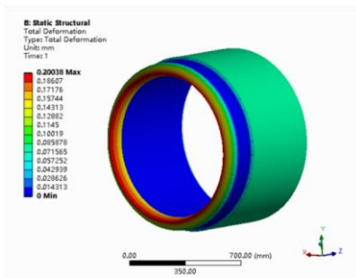
Figure 8: Thermal deformation of the guide sleeve
