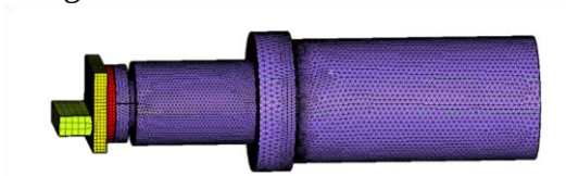
Figure 6: The whole model meshing
