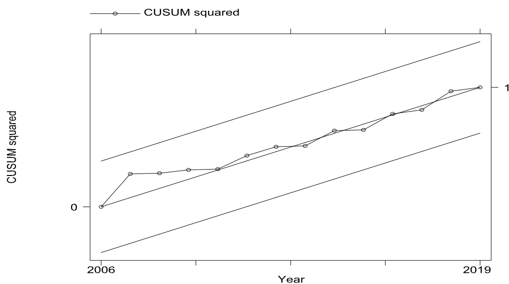
Figure 2. CUSUM squared. Source: Authors.
