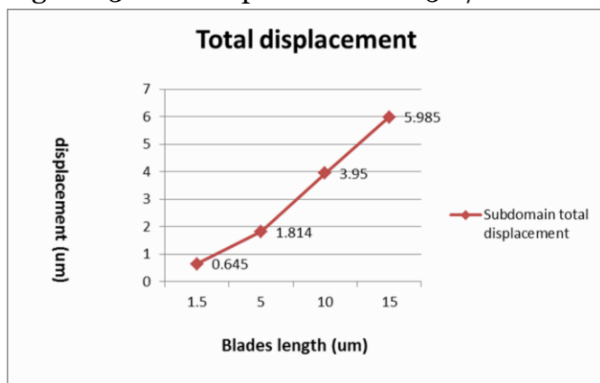
Figure 13 Total displacement in 15m/s maximum inlet speed in Case 4
